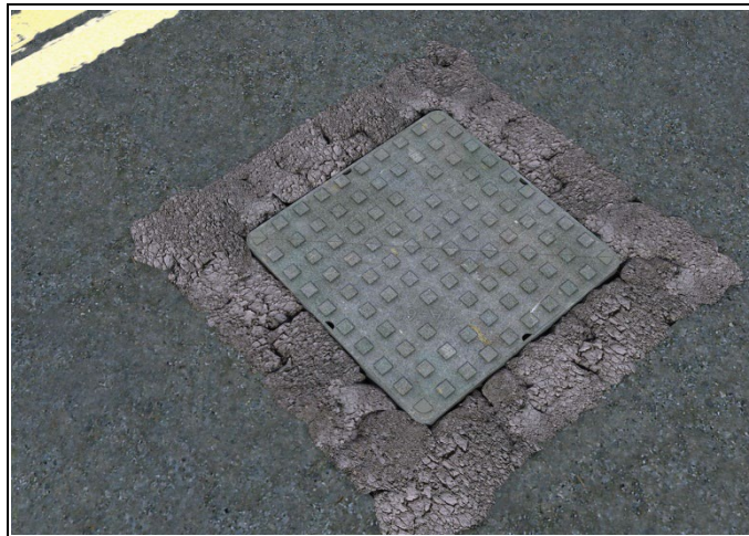
Figure 1 Failed ironwork
