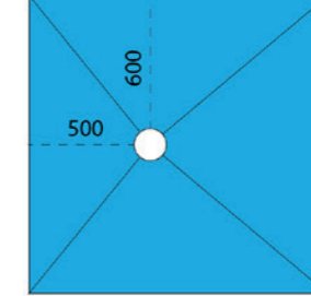
UT PDeck 103 SQ 1200 x 1200 x 22mm
