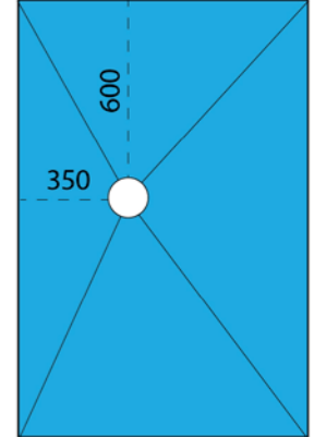
UT PDeck 108 SQ 1400 x 900 x 22mm
