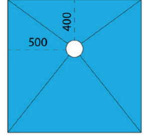
UT PDeck 104 SQ 1000 x 1000 x 22mm
