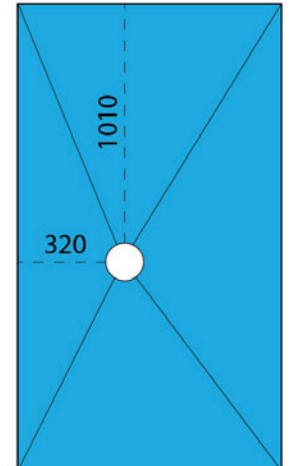
UT PDeck 112 SQ 1800 x 800 x 22mm
